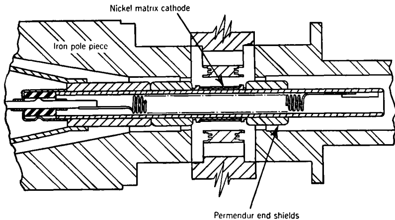
FIG. 12-32.—Oxide matrix cathode of the 4J50. (2X)
